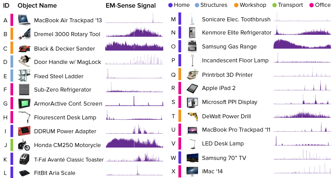
Figure 4-9. EM spectrums (0Hz - 1MHz) for the evaluation, captured by the
