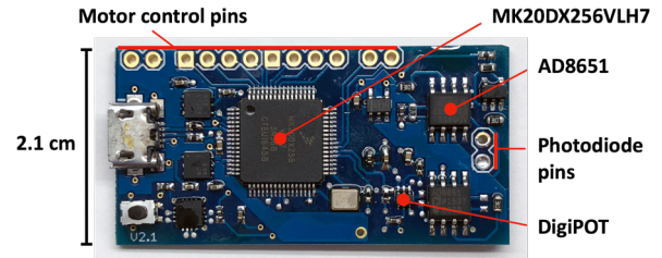
Figure 9. Vibrosight driver/sensor board.
